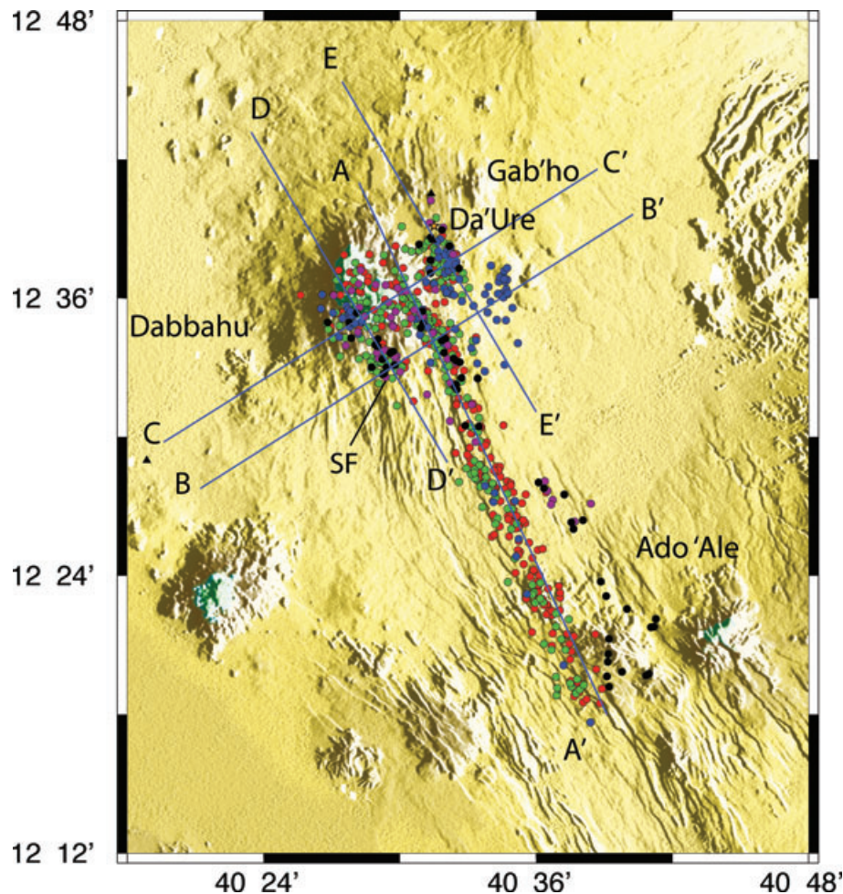
Figure 4. Earthquake epicentres relocated using the double difference method of Waldhauser & Ellsworth (2000). A-A', B-B', C-C', D-D', E-E' mark the locations of topography and seismicity profiles shown in Figs 7 and 8. Colours signify temporal variations: red, 2005 October 19–31; green, 2005 November 1–30; blue, 2005 December 1–31; violet, 2006 1–31; black, 2006 February 1–March 30. Ado 'Ale, Dabbahu, Gab'ho are silicic volcanoes.
